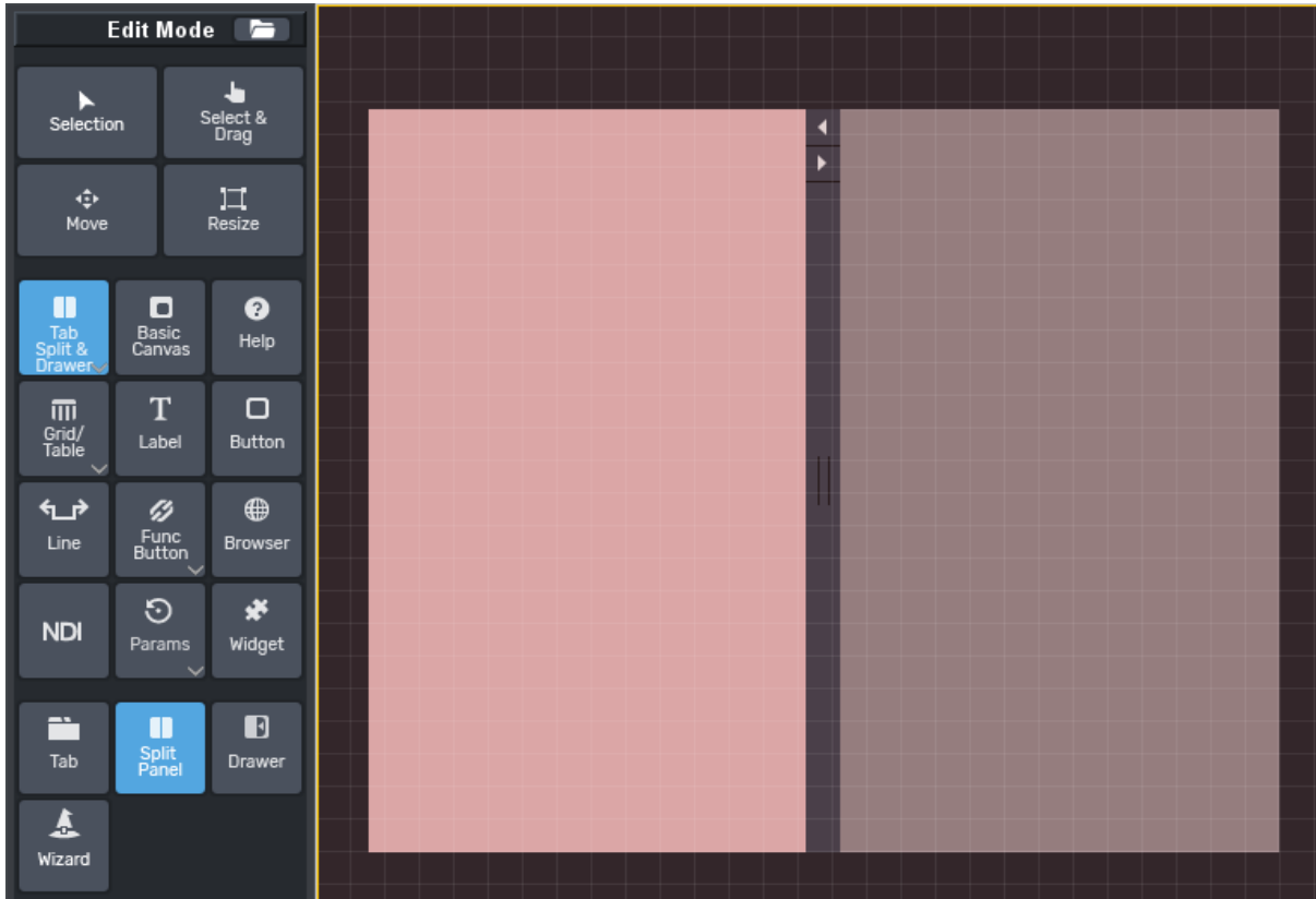
Figure 5.26 - Adding a Split Panel
