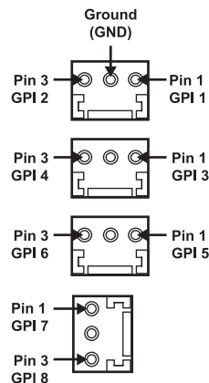
Figure 2.8 8320AR-033 GPI Connections
