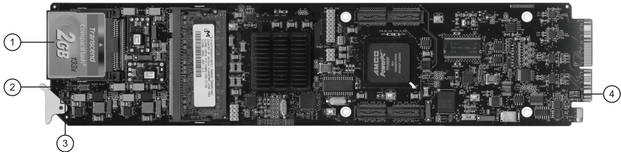
Figure 2.1 Card-edge Components
