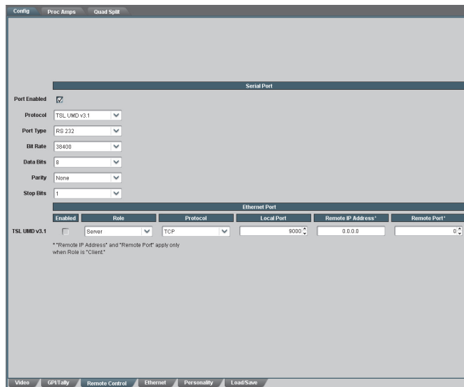
Config Tab — Remote Control Tab
