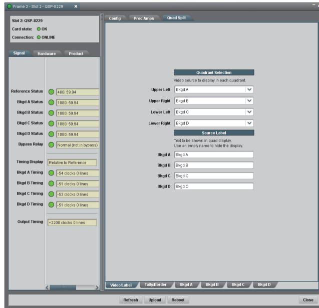
Quad Split — Video/Label Tab
