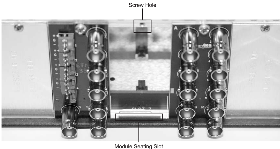
Figure 2.1 Rear Module Installation in a DFR-8300 Series Frame (GPI-100 not shown)
