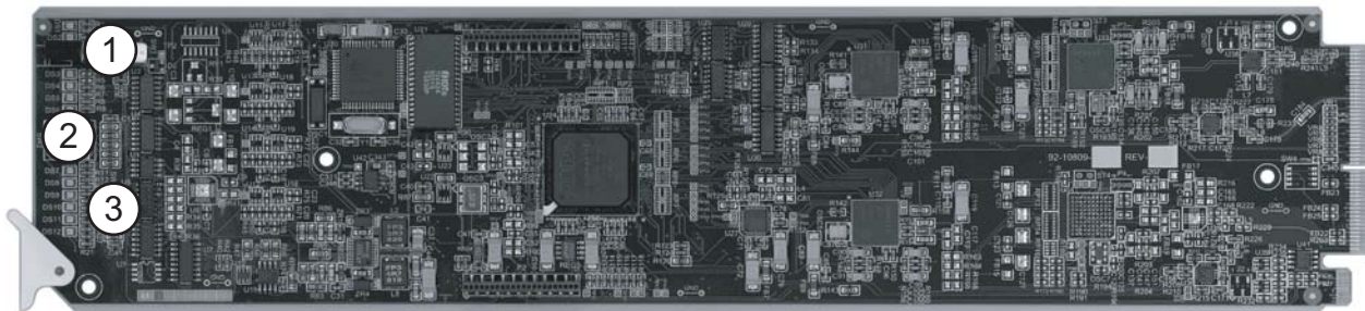
Figure 3.1 GPI-100 — Components
