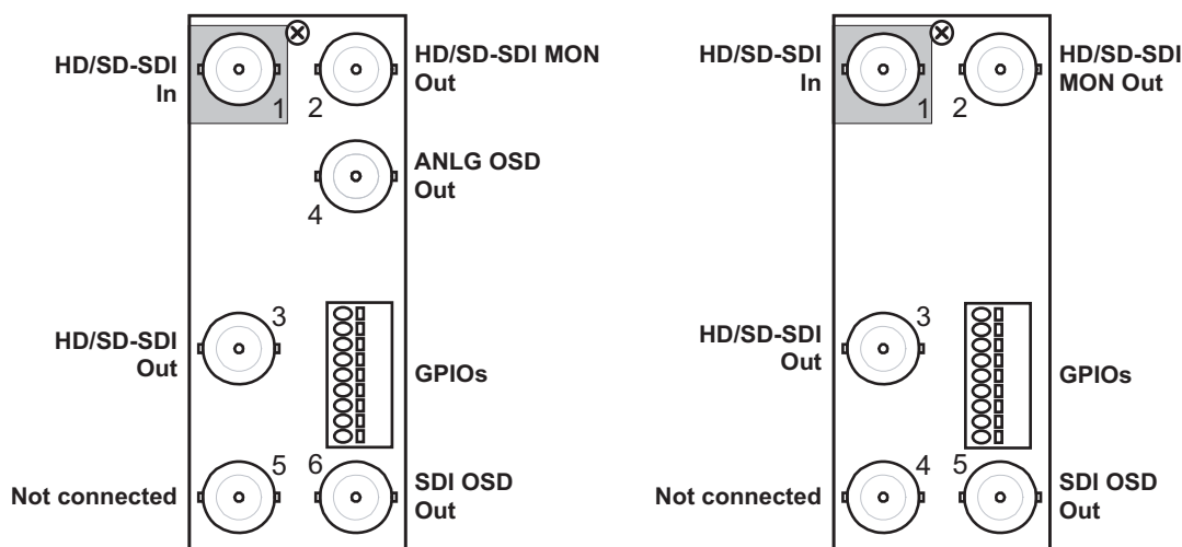
Figure 2.2 Cabling for the MDL-R10 Rear Module Figure 2.3 Cabling for the MDL-R20 Rear Module
