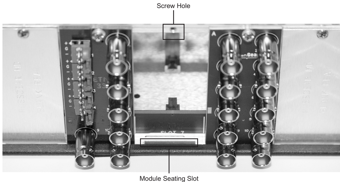
Figure 2.1 Rear Module Installation in a DFR-8310 Series Frame (ADC-8732B not shown)
