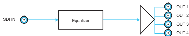
Figure 1.3 Simplified Diagram — 1x4 Configuration (8320AR-301)
