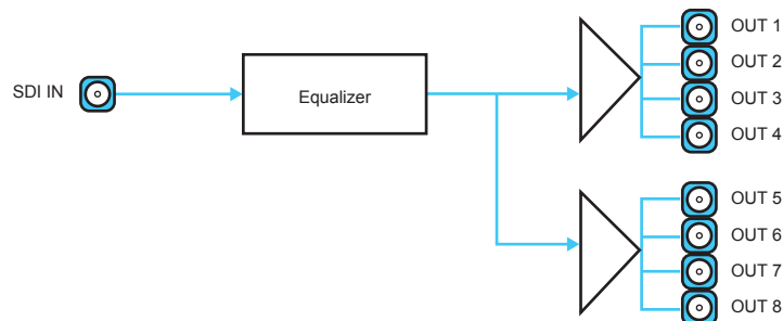
Figure 1.2 Simplified Diagram — 1x8 Configuration (8320AR-302)
