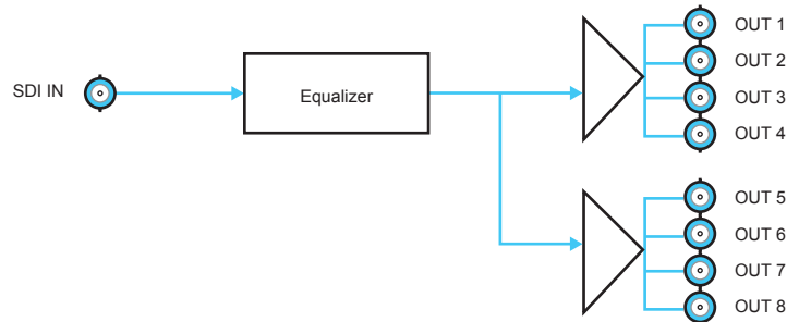
Figure 1.1 Simplified Diagram — 1x8 Configuration (8320AR-300)
