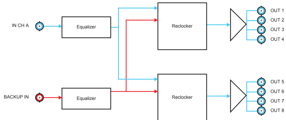
Figure 1.4 Simplified Diagram — Single 1x8 Configuration (8320AR-300)
