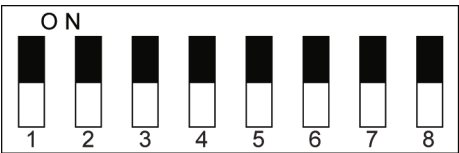
Figure 5. DIP Switch Positions (Off)
