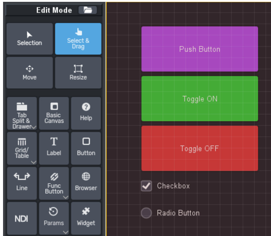
Figure 5.32 - Adding Buttons
