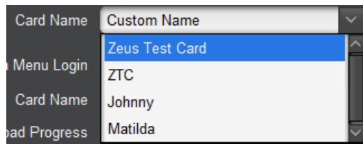
Figure 3.46 - WIDGET_COMBO_ENTRY Hint
