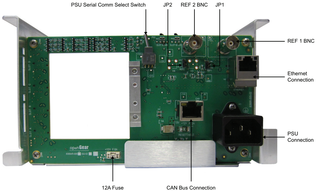
Figure 5.1 OTF-OGX Connections
