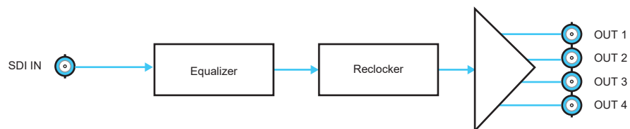
Figure 1.3 Simplified Diagram — 1x4 Configuration (8320AR-301)
