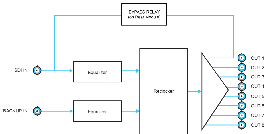
Figure 1.2 Simplified Diagram — 1x8 Configuration (8320AR-306)
