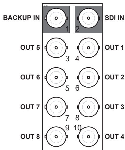
Figure 2.3 Cable Connections for 8320AR-306 Full Rear Module
