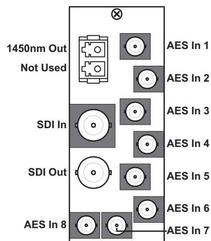
Figure 2.11 MUX-6258-A-45
