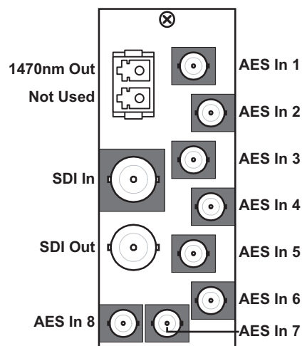
Figure 2.12 MUX-6258-A-47
