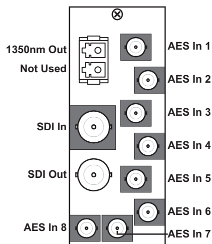
Figure 2.8 MUX-6258-A-35
