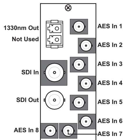
Figure 2.7 MUX-6258-A-33
