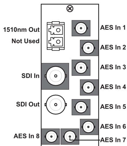
Figure 2.14 MUX-6258-A-51
