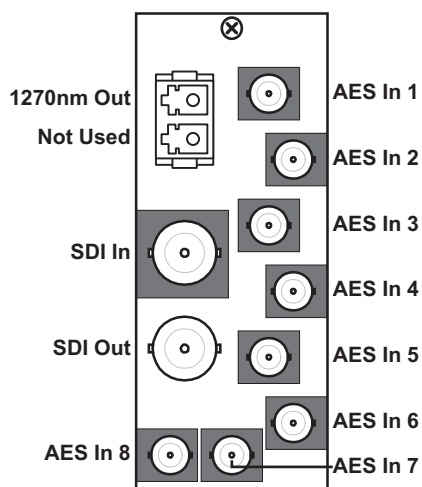
Figure 2.4 MUX-6258-A-27
