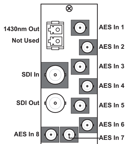
Figure 2.10 MUX-6258-A-43
