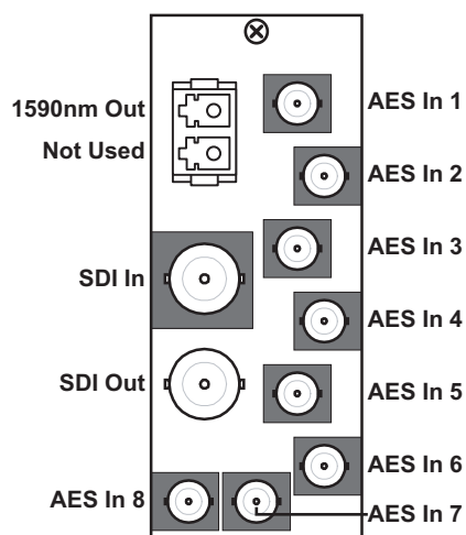
Figure 2.18 MUX-6258-A-59
