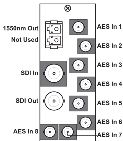
Figure 2.16 MUX-6258-A-55
