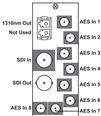
Figure 2.6 MUX-6258-A-31
