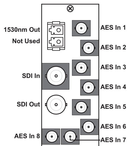
Figure 2.15 MUX-6258-A-53
