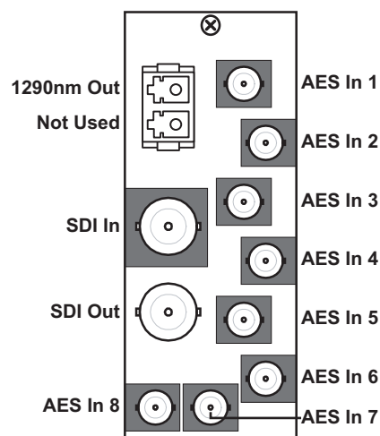
Figure 2.5 MUX-6258-A-29
