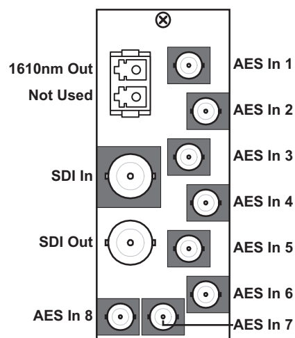
Figure 2.19 MUX-6258-A-61
