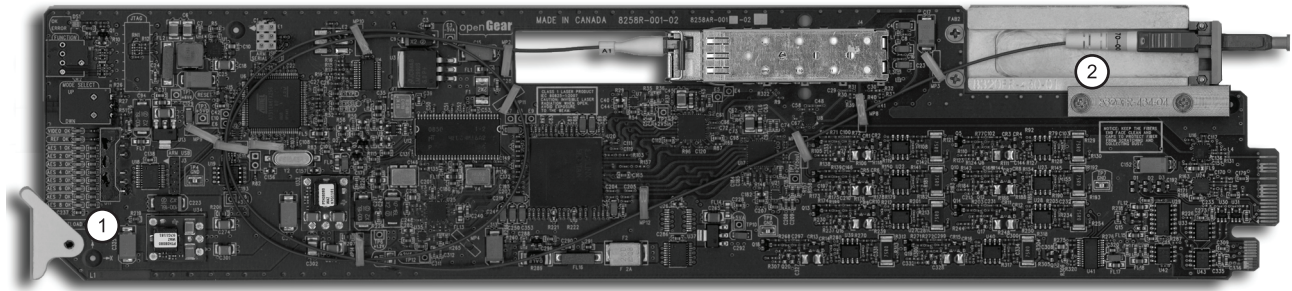
Figure 3.1 MUX-6258-A — Card-edge Components
