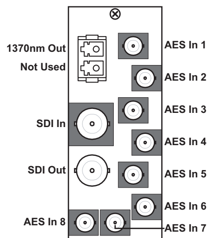
Figure 2.9 MUX-6258-A-37
