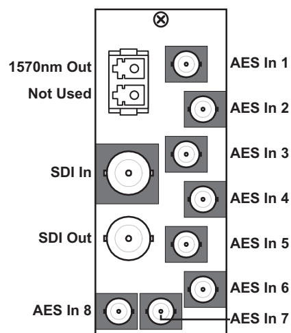
Figure 2.17 MUX-6258-A-57
