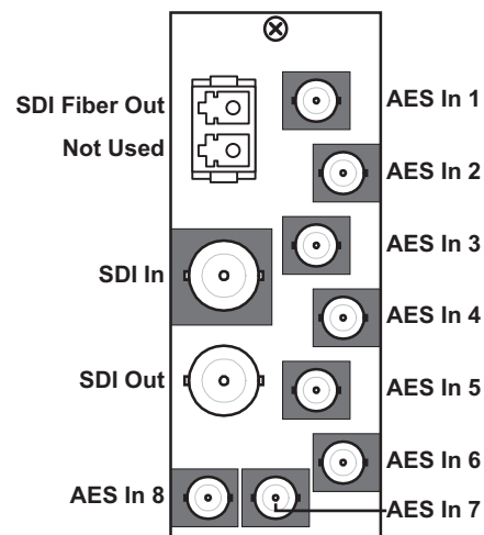
Figure 2.3 Cable Connections for the 8320AR-048A Rear Module
