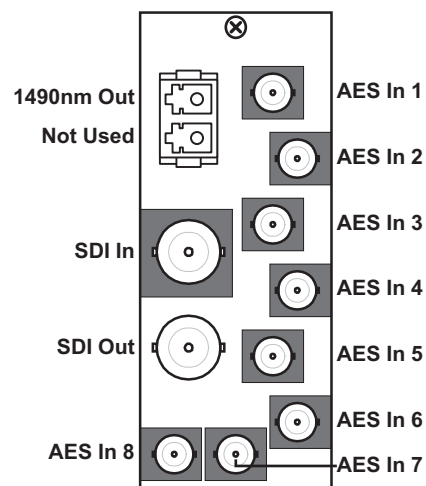
Figure 2.13 MUX-6258-A-49
