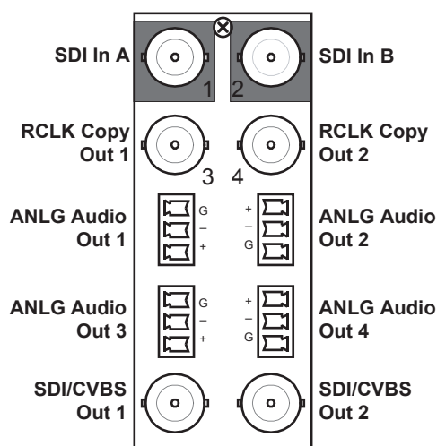
Figure 2.3 Cable Connections for the R2C-8223A Rear Modules
