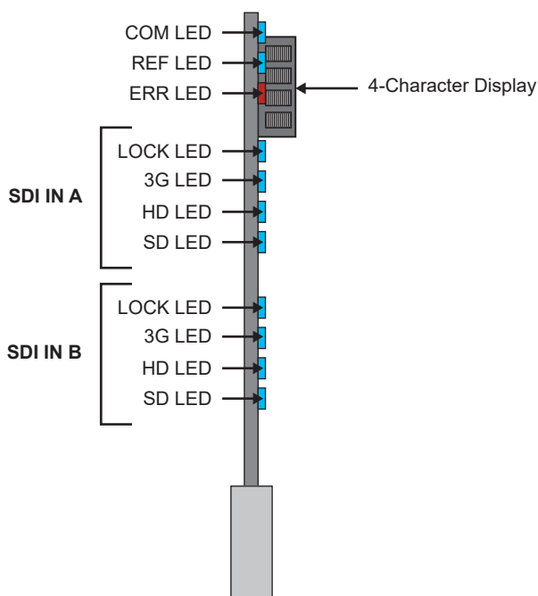
Figure 3.1 HDC-8223A(-S) Card-edge Controls
