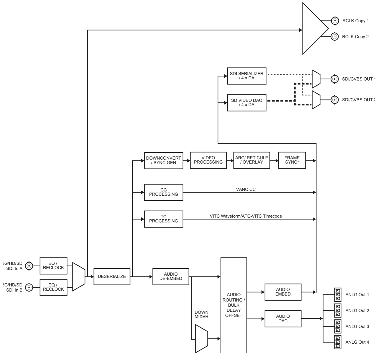
Figure 1.4 Functional Block Diagram — R2C-8223A Rear Module
