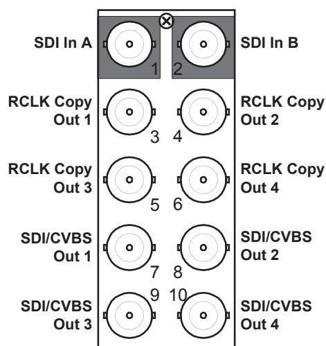
Figure 2.2 Cable Connections for the R2-8223A Rear Modules
