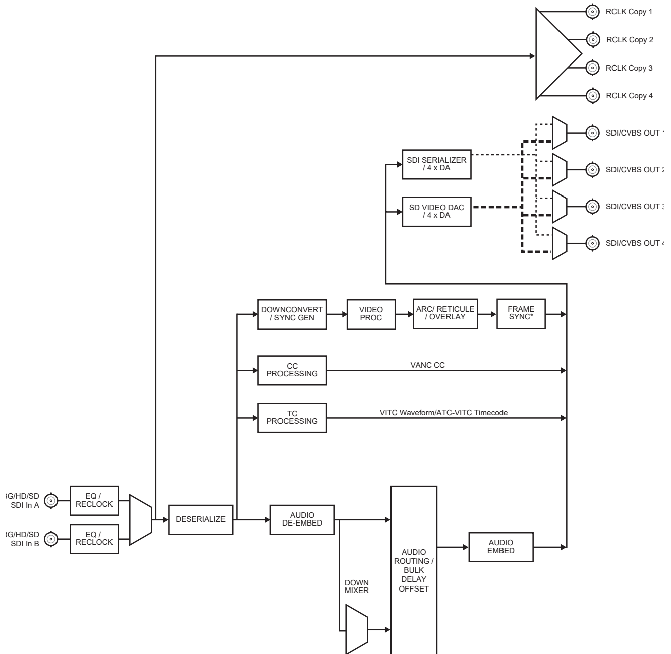
Figure 1.3 Functional Block Diagram — R2-8223A Rear Module
