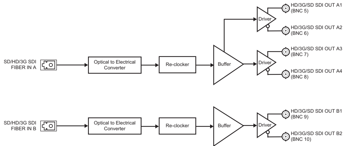
Figure 1.1 Simplified Block Diagram — 8320AR-044 Full Rear Module
