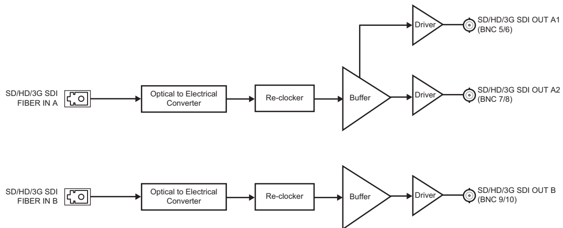
Figure 1.2 Simplified Block Diagram — 8320AR-045 Split Rear Module (Single Card only)
