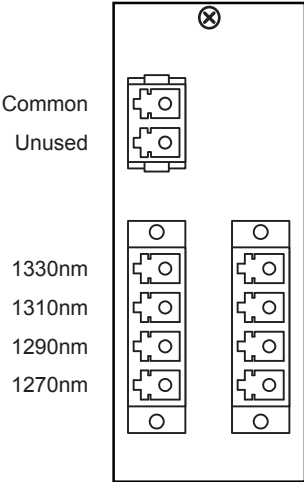
Figure 2.3 Cable Connections for the FCM-6846 and FCD-6847
