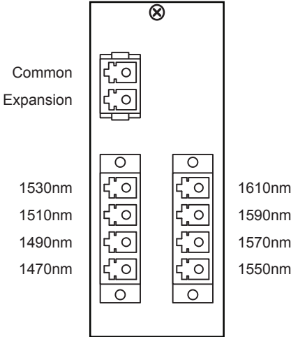
Figure 2.4 Cable Connections for the FCM-6848 and FCD-6849
