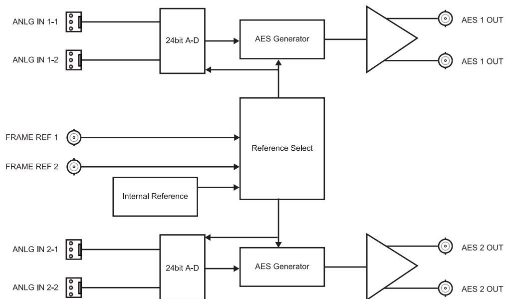
Figure 1.1 Simplified Block Diagram — 8310AR-036 and 8320AR-036 Full Rear Modules
