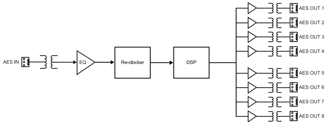
Figure 1.1 Simplified Block Diagram — 8310AR-042 and 8320AR-042 Full Rear Modules
