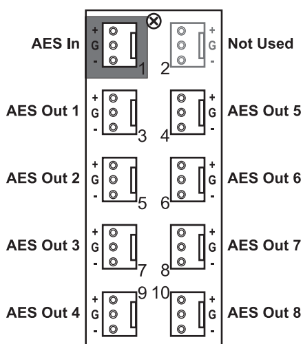
Figure 2.2 Cable Connections for the 8310AR-042 and 8320AR-042 Rear Modules
