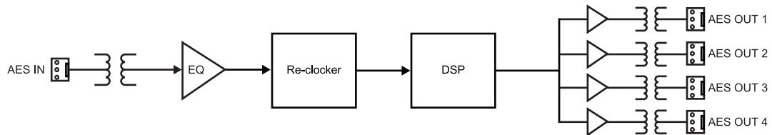
Figure 1.2 Simplified Block Diagram — 8320AR-043 Split Rear Module
