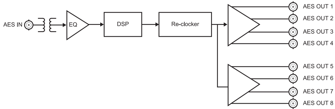
Figure 1.1 Simplified Block Diagram — 8310AR-030 and 8320AR-030 Full Rear Modules
