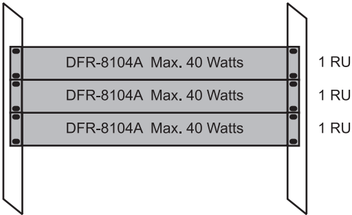
Figure 2.2 Frame Stacking — CFM-8104A Installed
