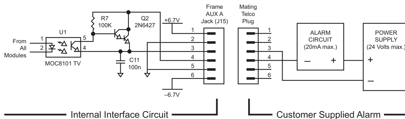
Figure 2.4 SMPTE 269M Alarm Reporting Internal Interface and Typical Connections
