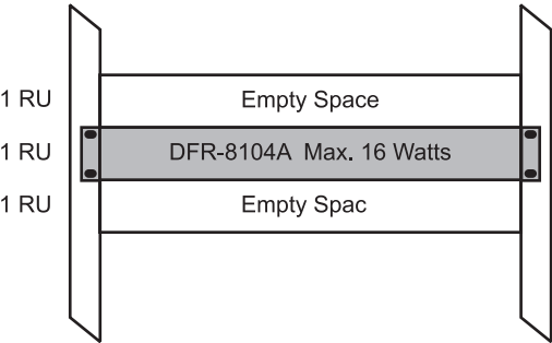
Figure 2.1 Frame Stacking — CFM-8104A Not Installed
