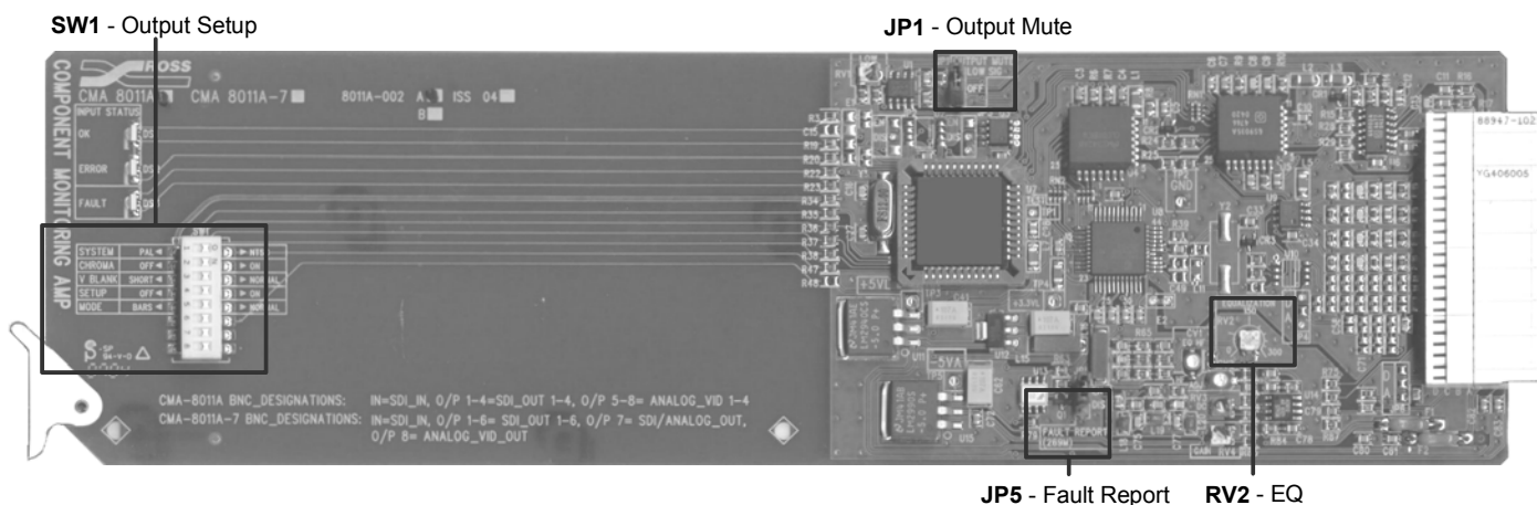
Figure 2. User Control Locations
