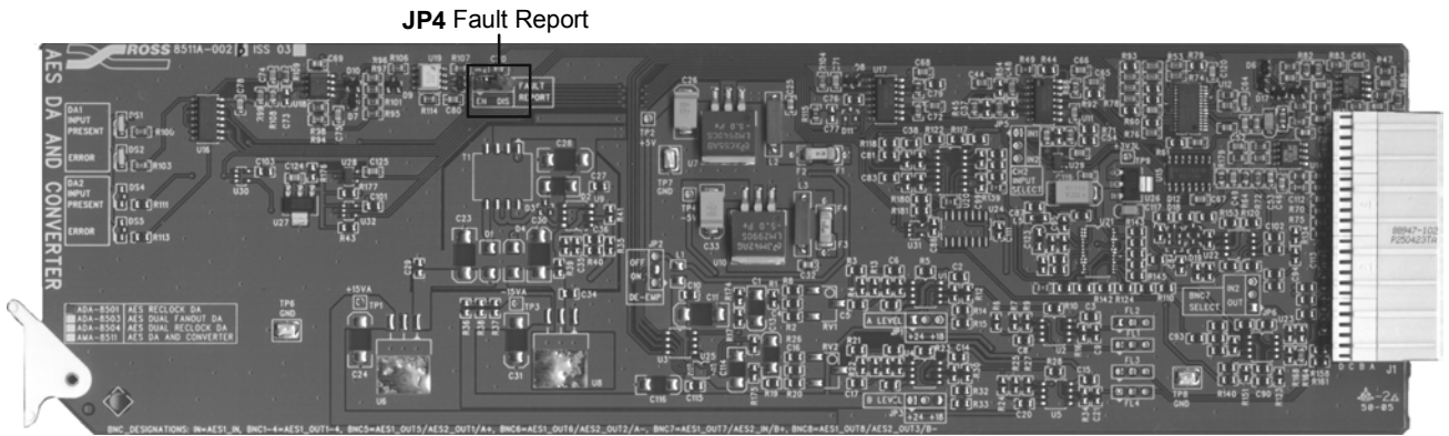
Figure 2. Jumper Locations
