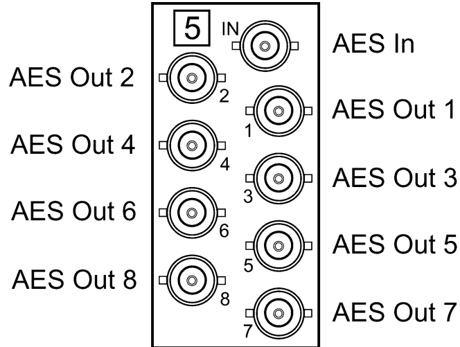
Figure 3. ADA-8501 BNC Designations for RossGear DFR-8110A (2RU frame)
