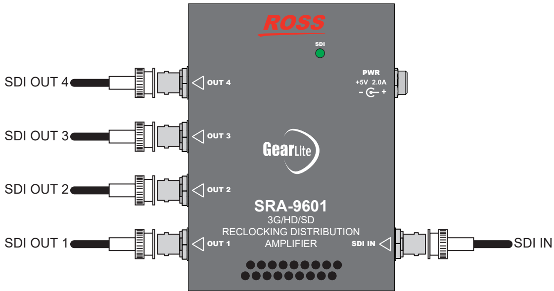
Figure 5.1 SRA-9601 — SDI Connections
