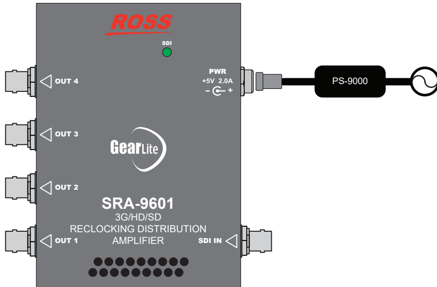
Figure 5.2 SRA-9601 — Power Connection
