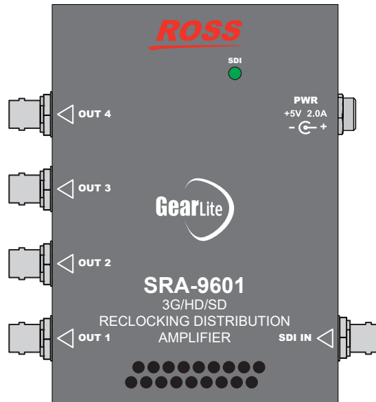
Figure 3.1 SRA-9601 — Faceplate Label
