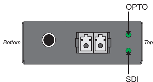
Figure 5.6 FDB-9649-LC (Right) — OPTO Status LEDs
