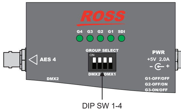
Figure 3.7 DMX-9259-A — DIP Switch Locations
