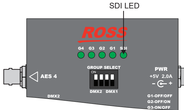
Figure 3.6 DMX-9259-A — SDI LED
