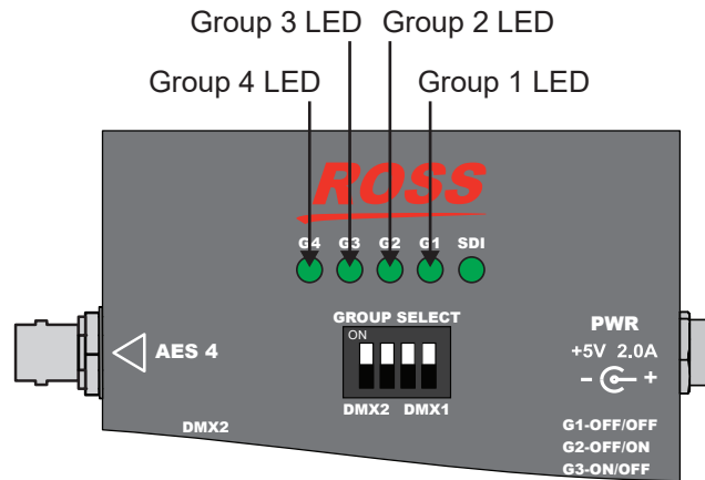
Figure 3.4 DMX-9259-A — Audio Group LEDs
