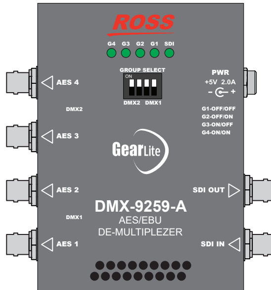
Figure 3.1 DMX-9259-A — Faceplate Label
