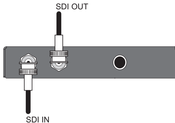
Figure 5.2 DMX-9259-A — SDI Connections
