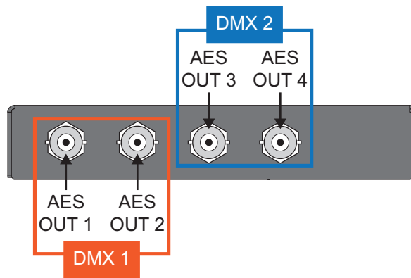
Figure 3.3 DMX-9259-A — AES Connections
