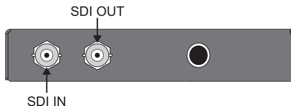
Figure 3.5 DMX-9259-A — SDI Connections
