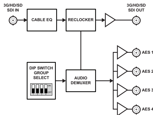
Figure 2.1 Simplified Block Diagram of DMX-9259-A Functions
