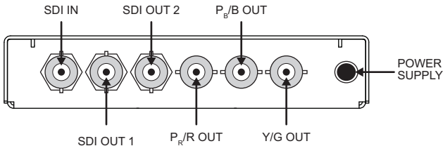
Figure 5 DAC-9213-R Connections
