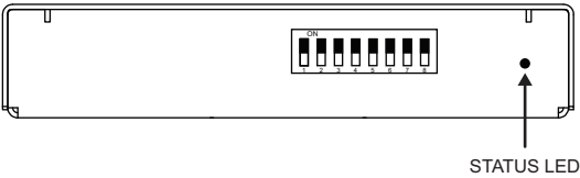
Figure 7 CMA-9011 Status Indicator LEDs
