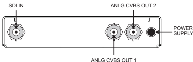
Figure 5 CMA-9011 Connections
