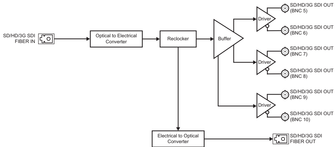
Figure 1.1 FSR-6605 with Full Rear Module (8320AR-044) — Simplified Block Diagram
