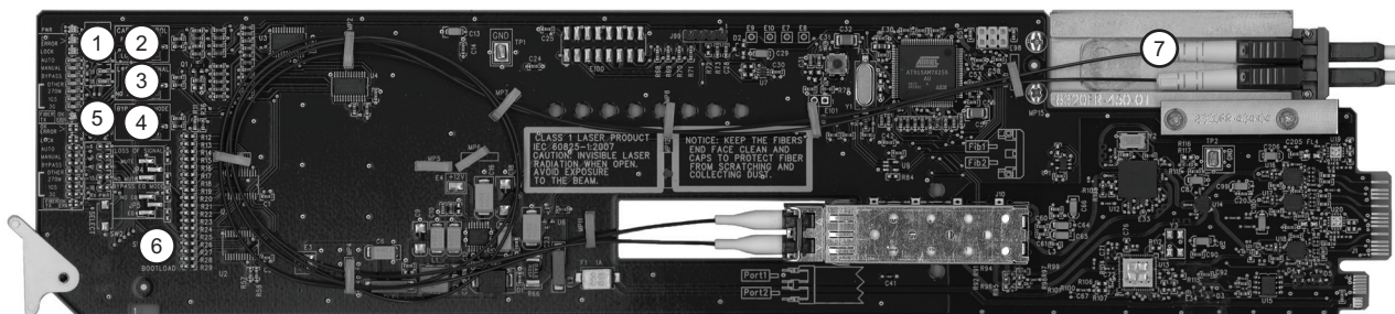
Figure 3.1 FSR-6605 — Components
