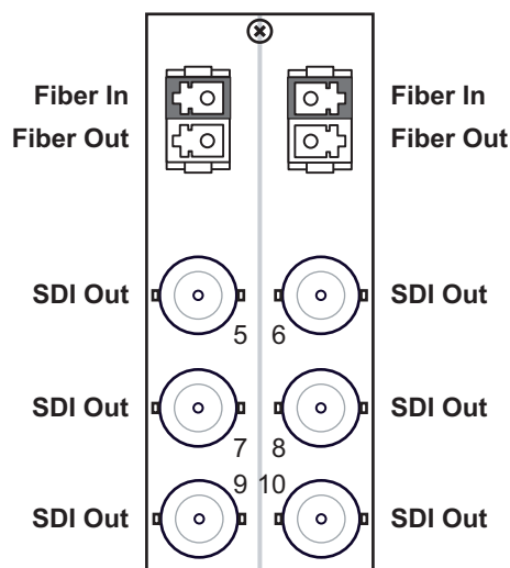
Figure 2.5 Cable Connections for the 8320AR-045 Rear Module
