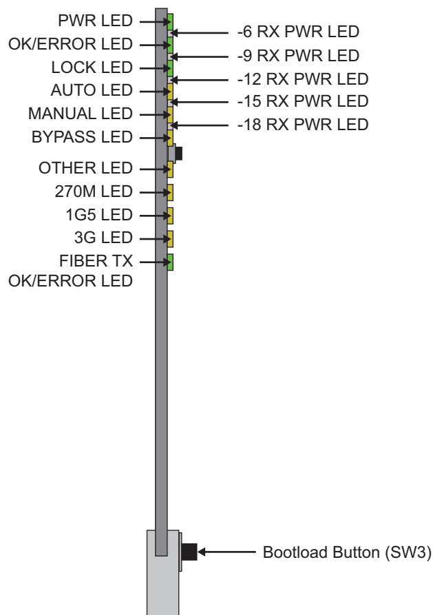
Figure 3.2 FSR-6605 Card-edge Controls
