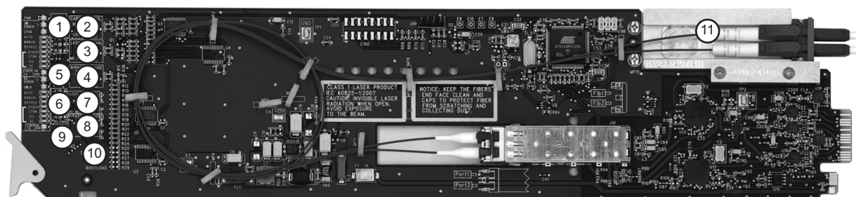
Figure 3.1 FDR-6603 — Components
