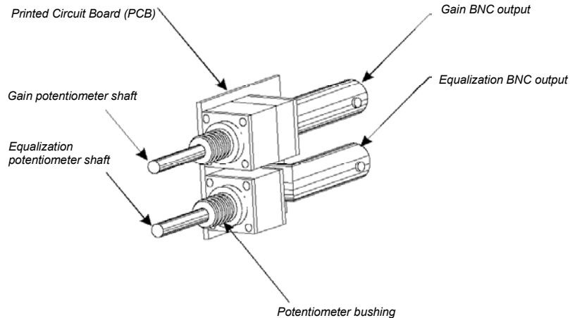
Figure 4. The Control Module PCB
