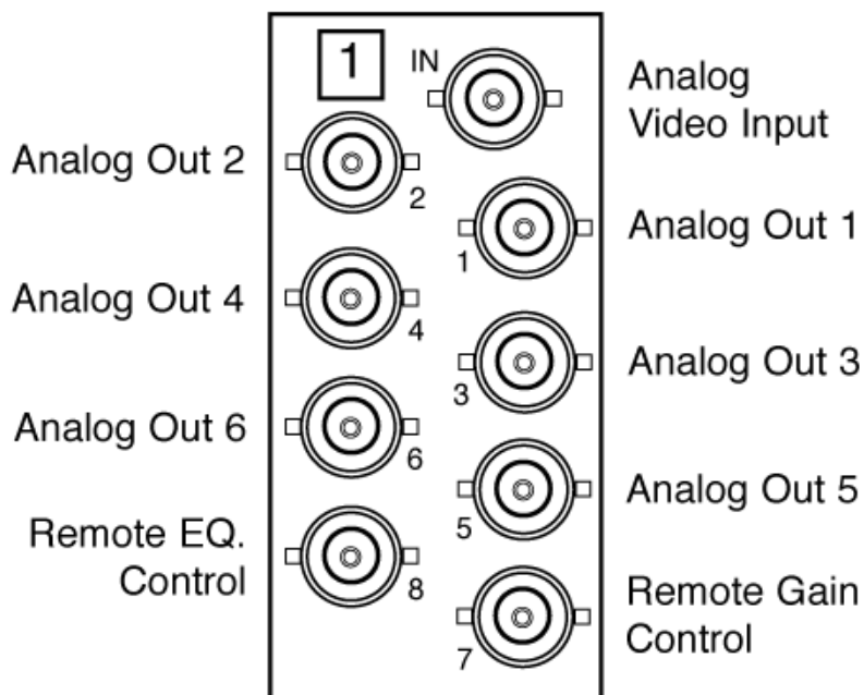
Figure 8. VTA-8060 Cabling Designations for RossGear 7200 and 7850 Series Frames
