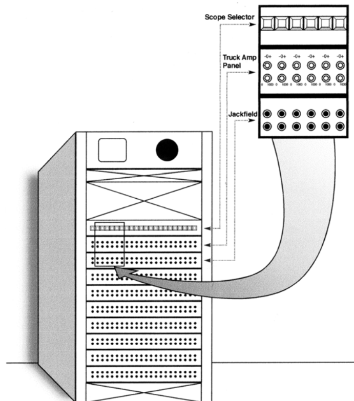
Figure 3. Truck Amp installed in equipment rack
