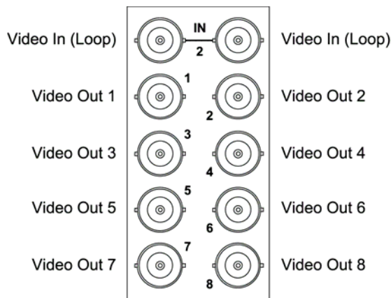
Figure 2. VEA-7007A Cabling Designations for RossGear 7200 and 7850 Series Frames
