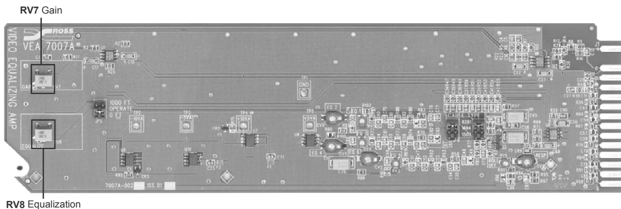
Figure 3. VEA-7007A Operational Setting Locations
