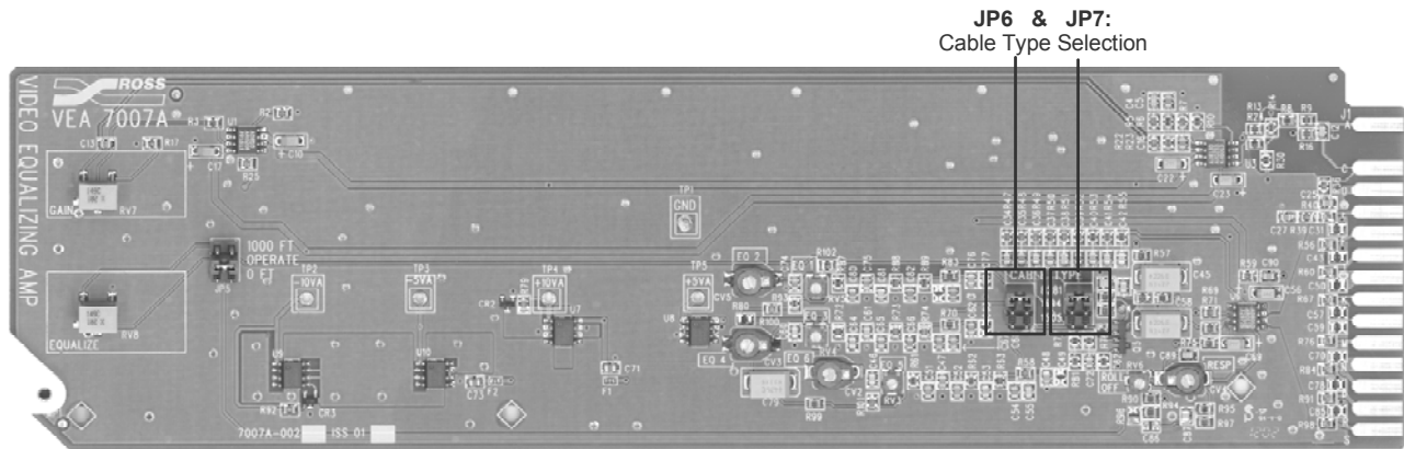
Figure 2. VEA-7007A Jumper Locations
