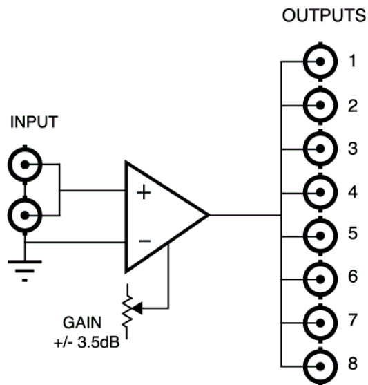
Figure 1. Simplified Block Diagram of UDA-7005A Functions
