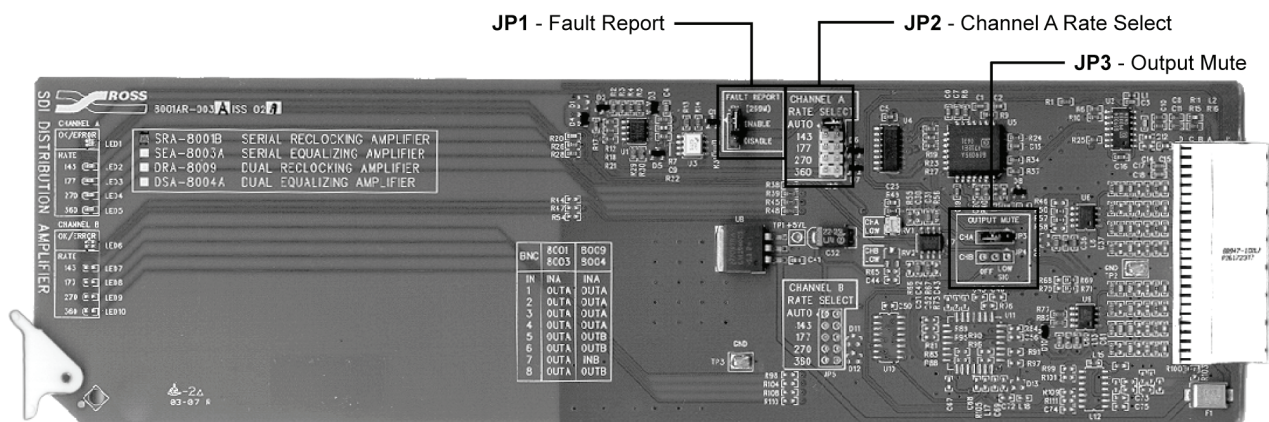
Figure 3. Jumper Locations
