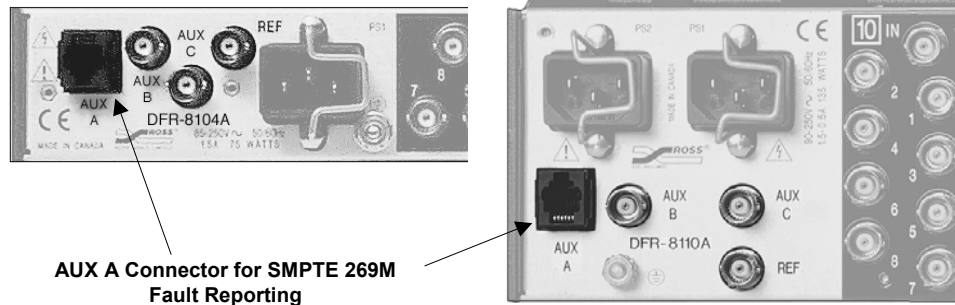
Figure 6. SMPTE 269M Alarm Reporting Frame Connections
