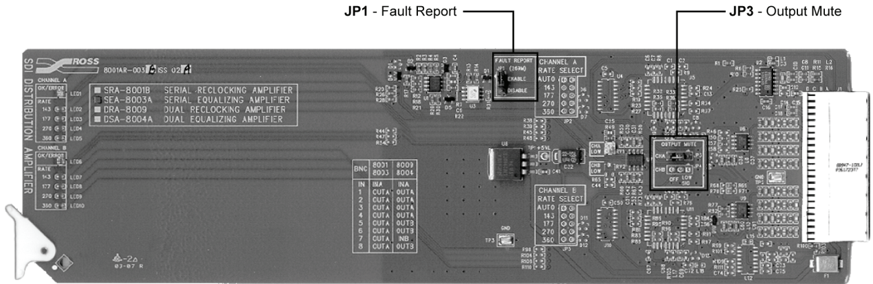
Figure 3. Jumper Locations
