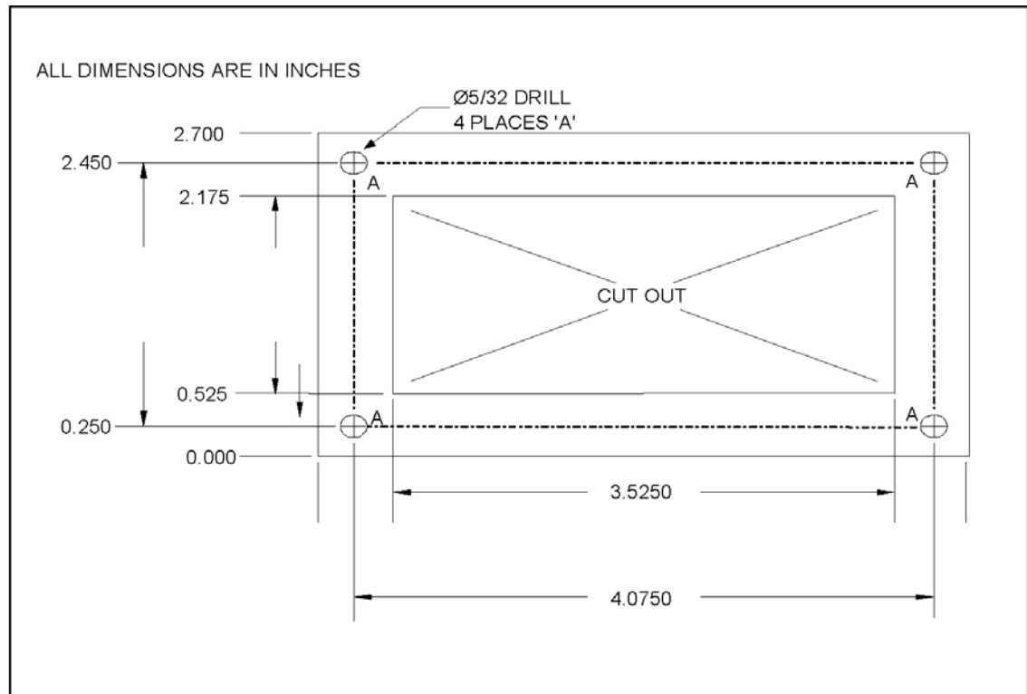
Figure 3. DCA-8120 In Desk Mounting Template.
