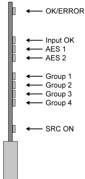
Figure 7. Card-edge LEDs
