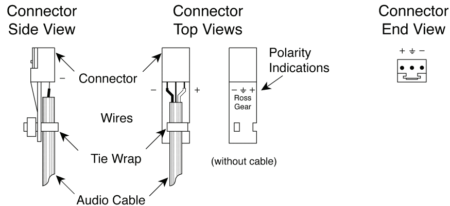
Figure 4. Connector Wiring for CON-8552 Input Sockets
