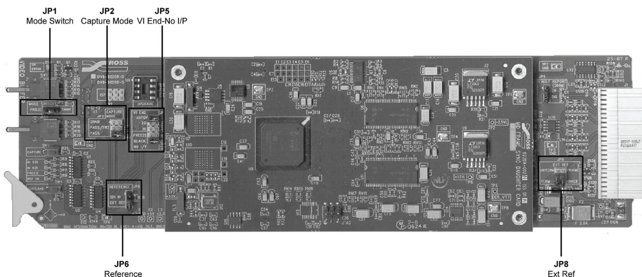
Figure 4. Jumper Locations
