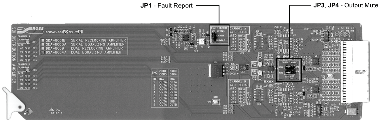
Figure 3. Jumper Locations
