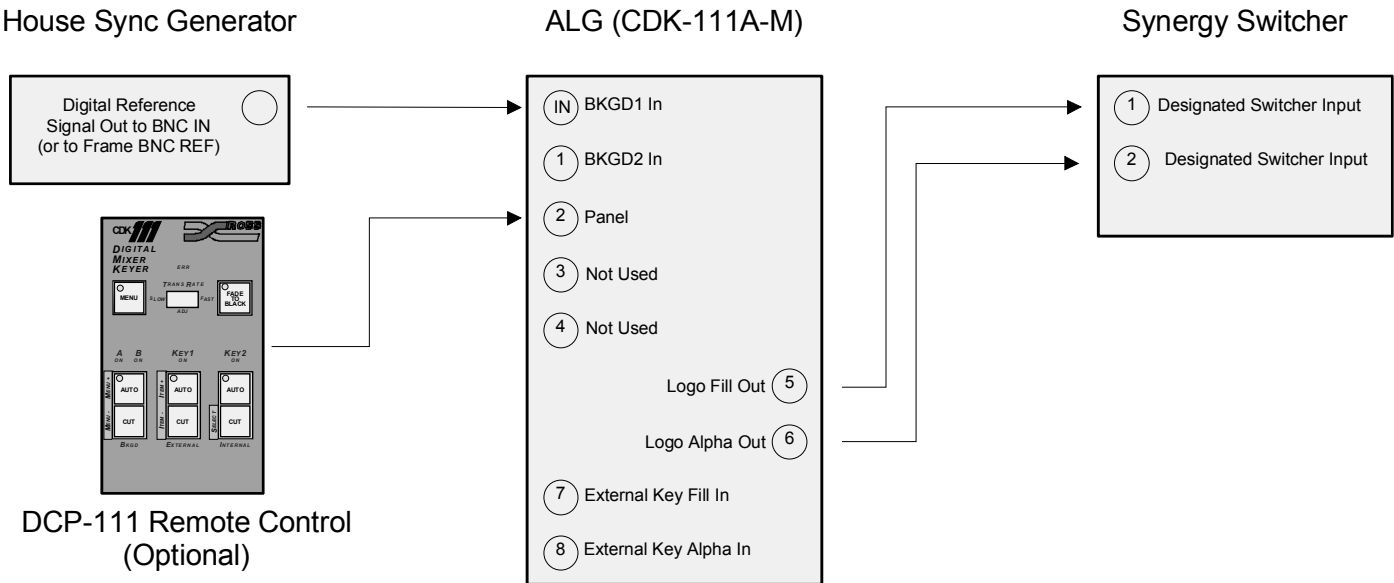
ALG (CDK-111A-M) Cabling Diagram
