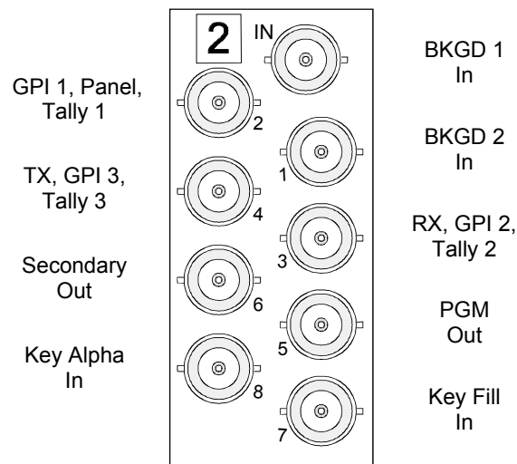
CDK-111A-M Connectors
