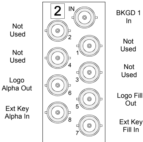
CDK-111A-M Connector Assignments
