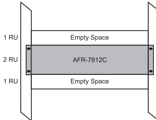
Figure 1.2 Frame Stacking
