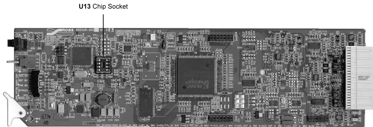
Figure 23. ADL-8520A Upgrade Socket and Label Locations
