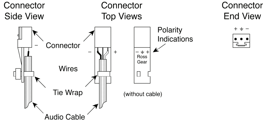
Figure 11. Connector Wiring for CON-8520-A
