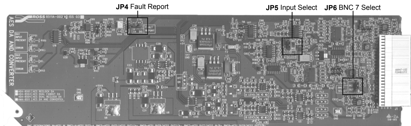
Figure 2. Jumper Locations
