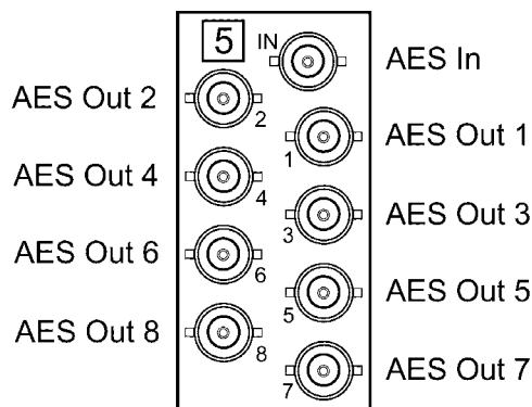
Figure 3. ADA-8503 BNC Designations for RossGear DFR-8110A (2RU frame)
