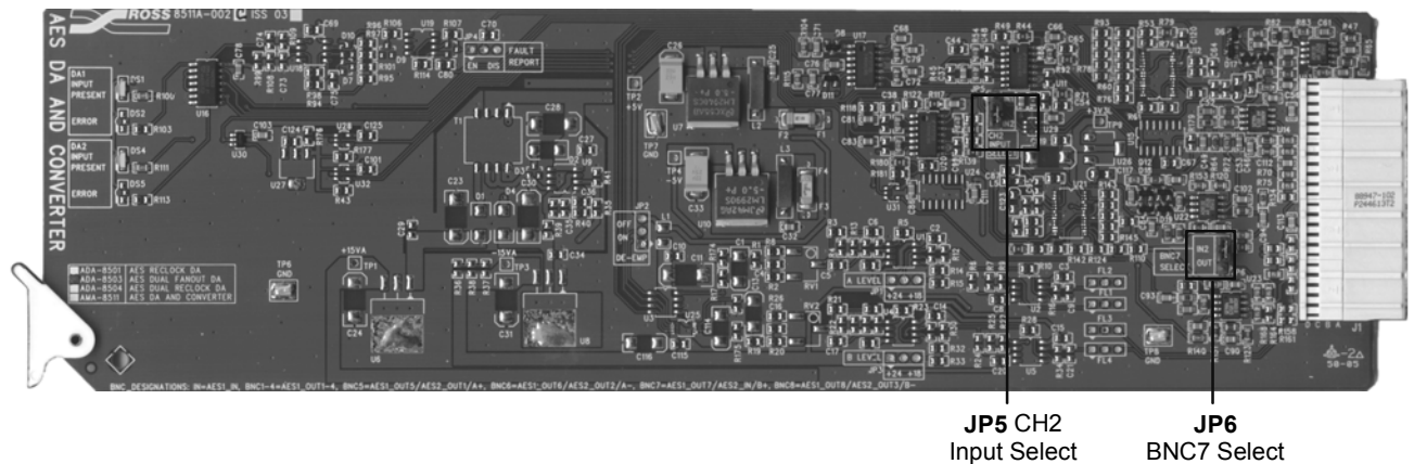
Figure 2. Jumper Locations
