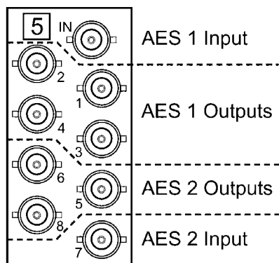
Figure 3. ADA-8503 BNC Designations for RossGear DFR-8110A (2RU frame)
