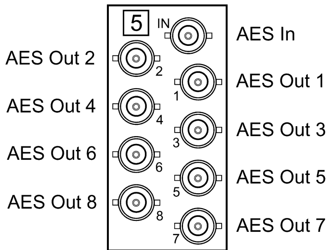
Figure 3. ADA-8501 BNC Designations for RossGear DFR-8110A (2RU frame)
