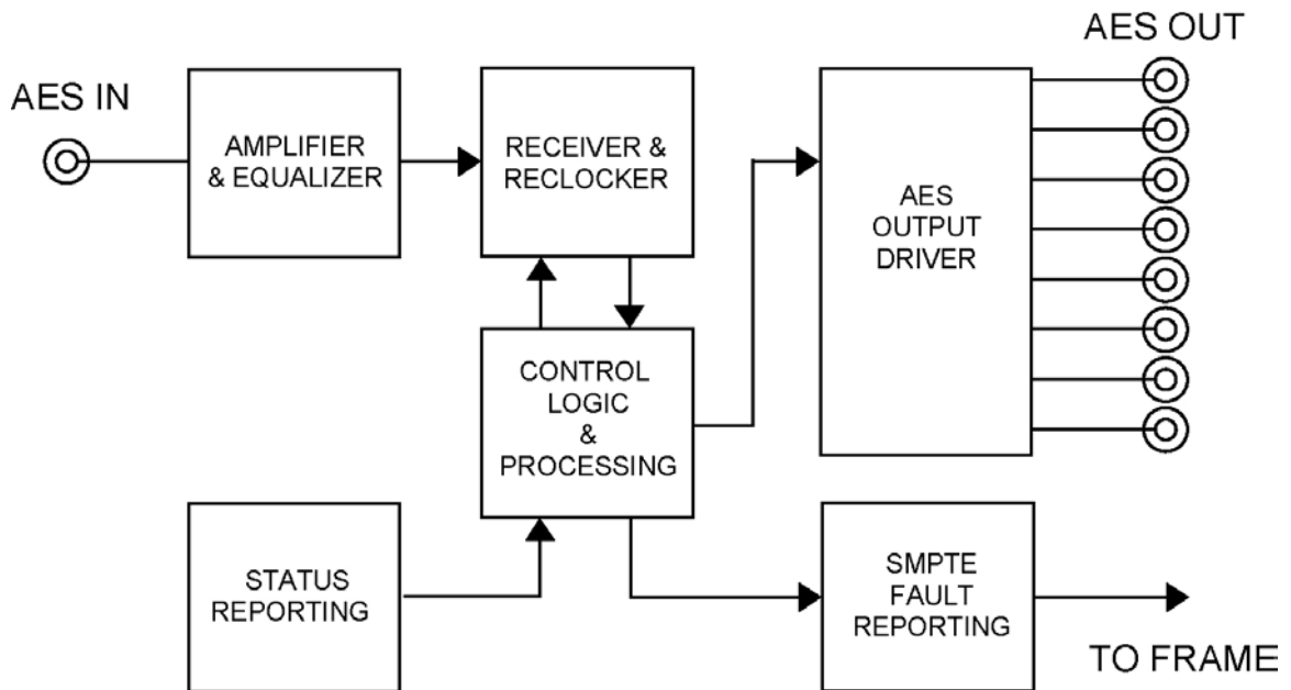
Figure 1. Simplified Block Diagram of ADA-8501 Functions
