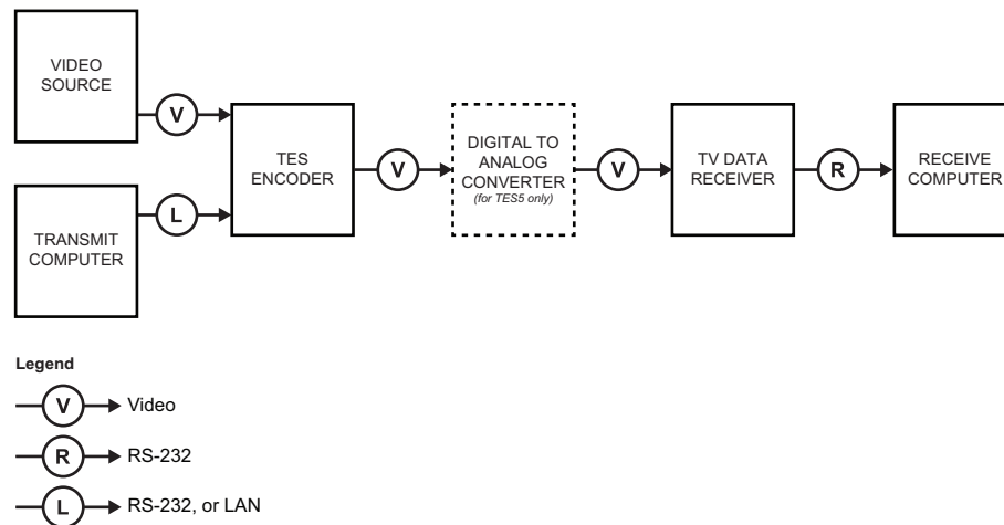
Figure 15.1 Setup Example
