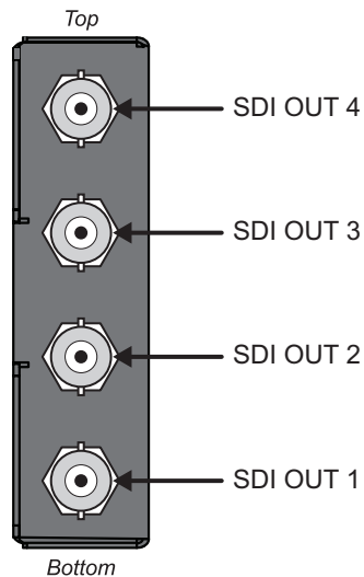
Figure 3.4 SRA-9601 — SDI Output Connections
