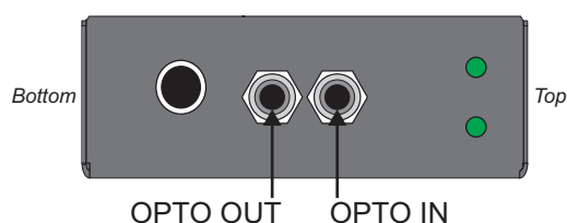
Figure 5.5 FDB-9649-ST (Bottom) — Fiber Optic Connections
