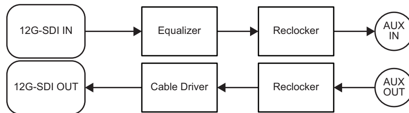
Figure 17 SFP-HDB-IO-12G — High Level Block Diagram
