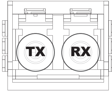
Figure 22 SFP Package Outline, Front View — Channel Position
