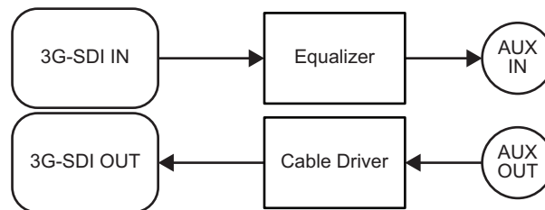
Figure 15 SFP-HDB-IO-3G — High Level Block Diagram
