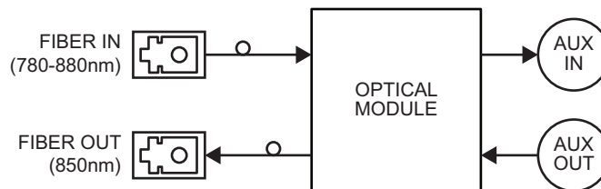
Figure 19 High Level Block Diagram
