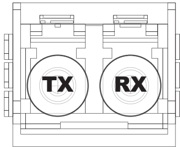
Figure 14 SFP Package Outline, Front View — Channel Position
