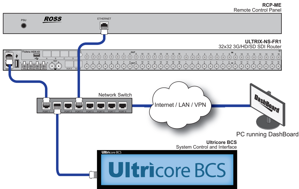
Figure 45 Example of a Simple Routing System with Ultrix and Ultracore BCS
