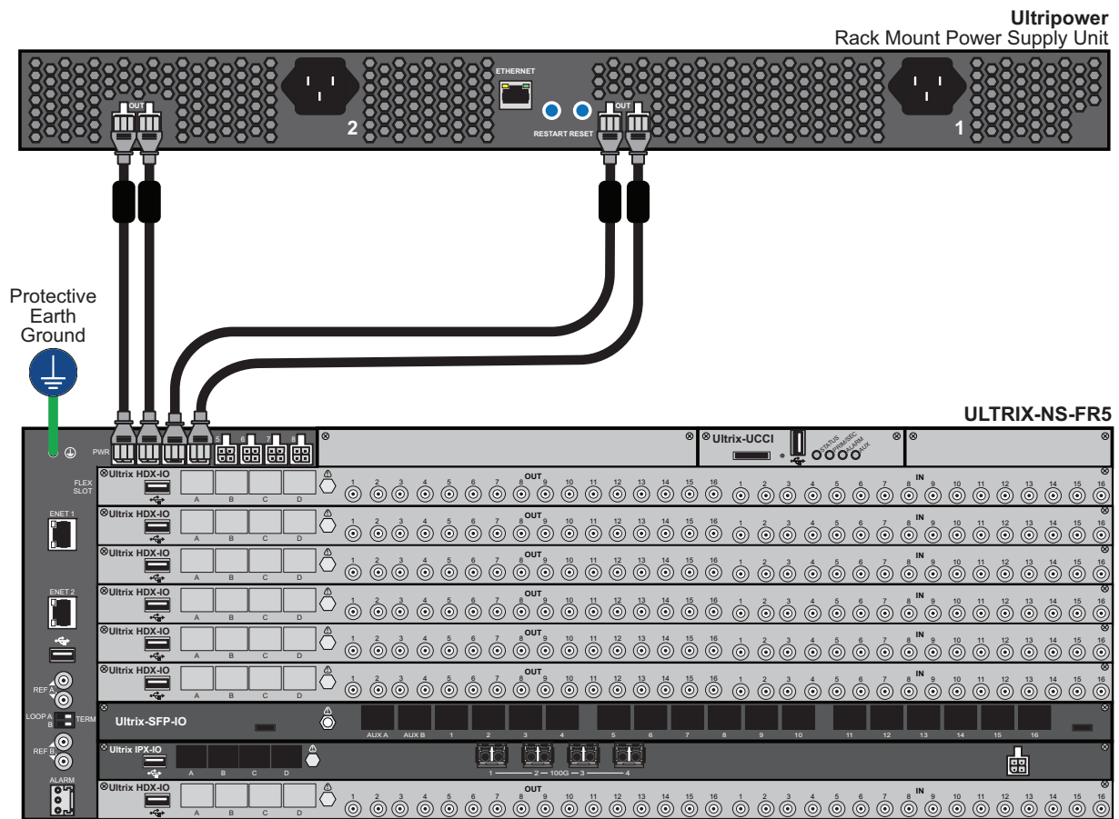
Figure 19 ULTRIX-NS-FR5 — Power Connections
