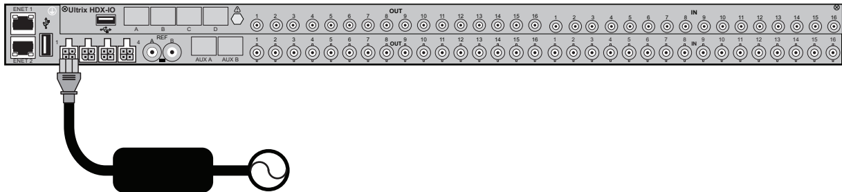
Figure 17 ULTRIX(-NS)-FR1 — Primary Power Connection
