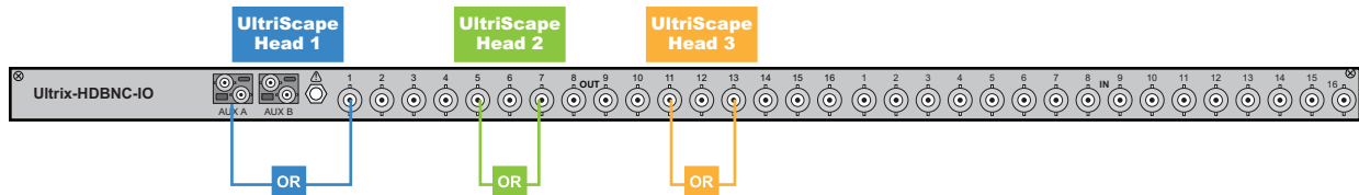
Figure 51 Ultrix Rear Panel — UltraScape Head Mapping for an ULTRIX-HDBNC-IO Blade
