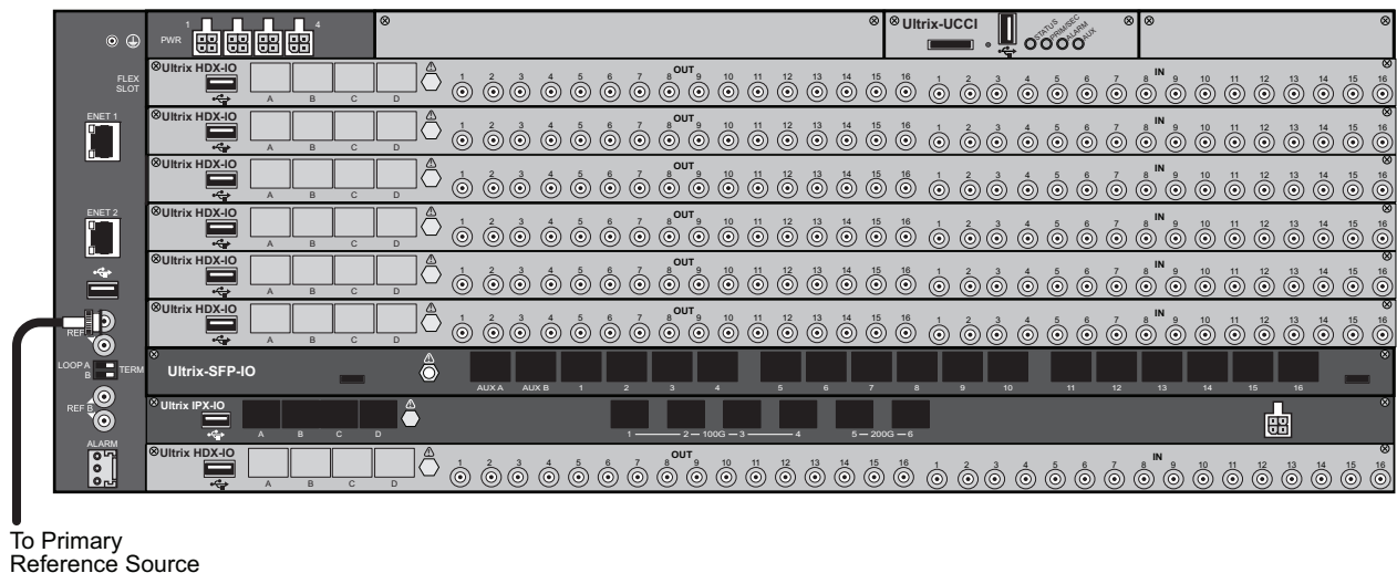
Figure 22 Video Reference Cabling — REF A Port on the ULTRIX-FR5
