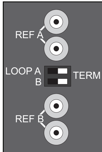
Figure 23 ULTRIX(-NS)-FR5 — DIP Switch in the TERM Positions
