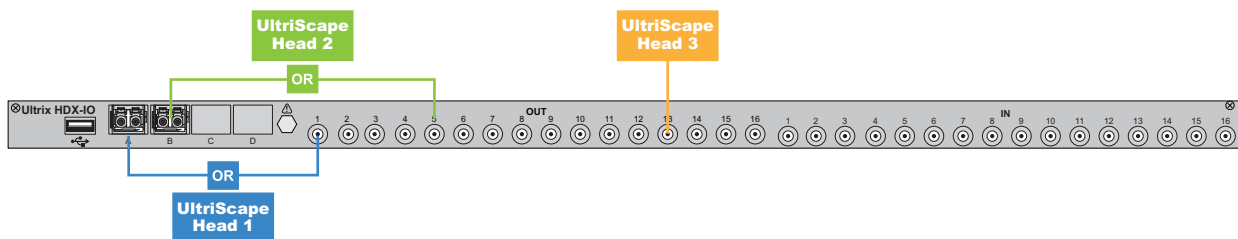
Figure 31 Example of Ultriscape Head Mapping on a Single ULTRIX-HDX-IO Blade
