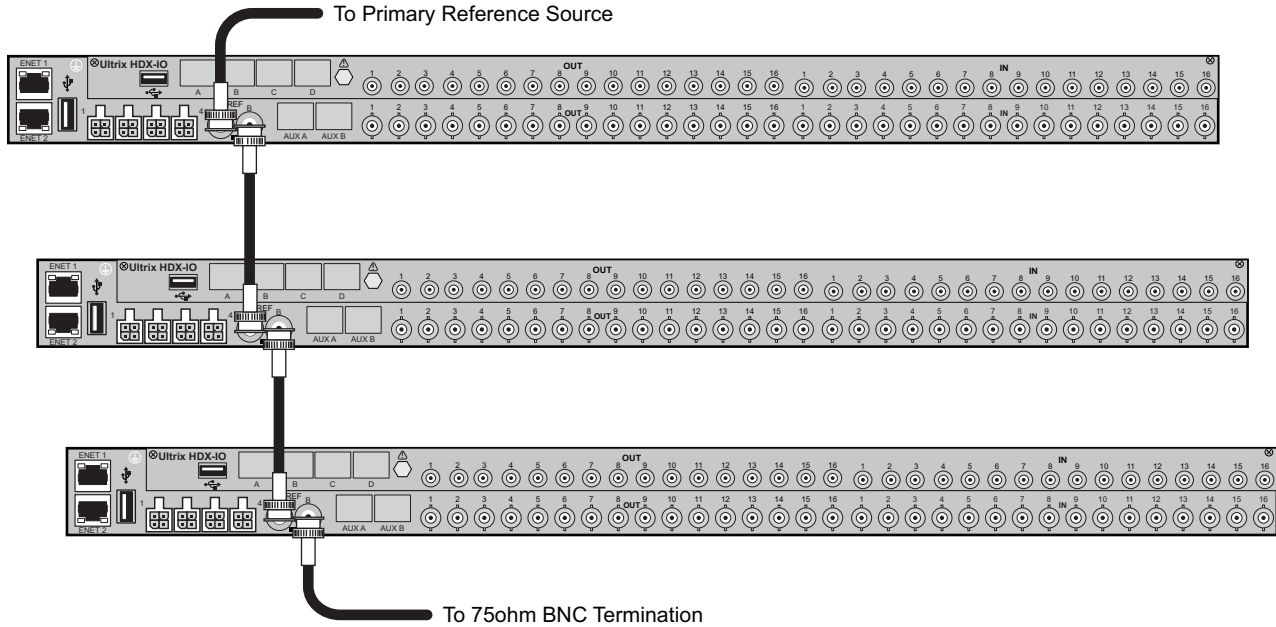
Figure 21 Connecting Multiple Routers for Simultaneous Switching
