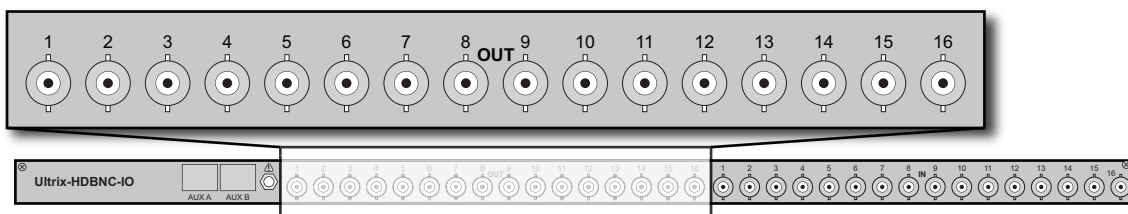
Figure 26 ULTRIX-HDBNC-IO Blade — SDI Outputs
