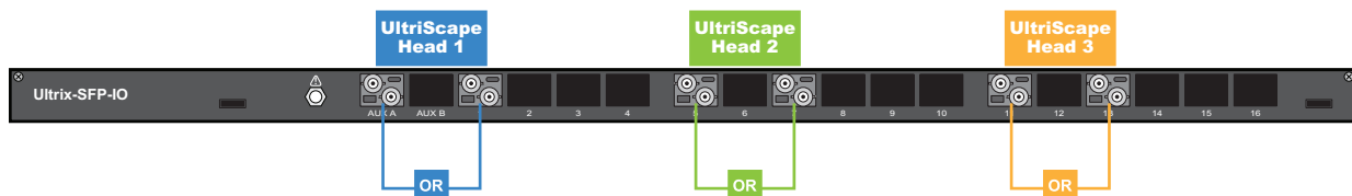
Figure 34 Example of Ultriscope Head Mapping on a Single ULTRIX-SFP-IO Blade
