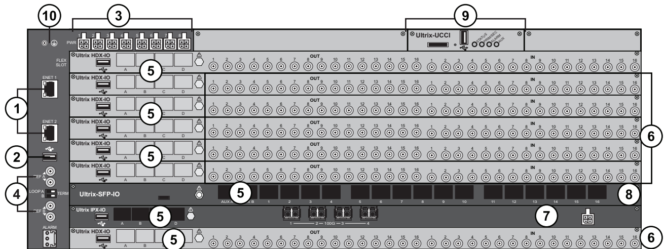
Figure 11 Rear Panel — ULTRIX-NS-FR5
