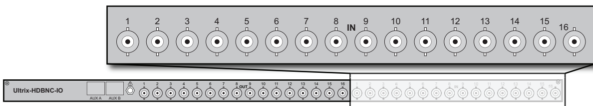
Figure 24 ULTRIX-HDBNC-IO Blade — SDI Inputs
