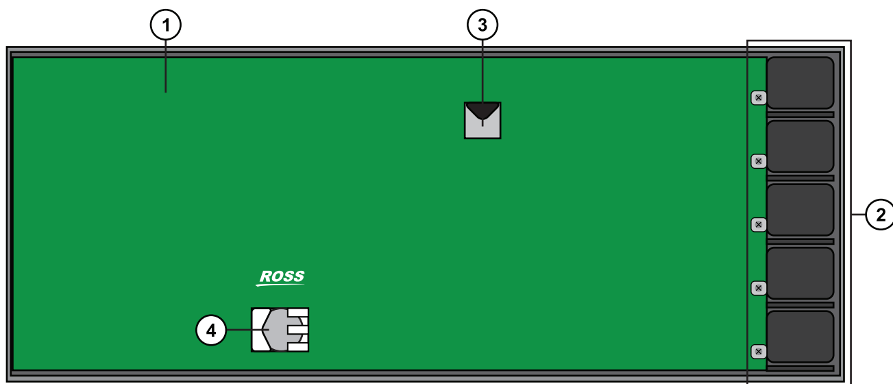
Figure 7 Overview of the Chassis Interior — ULTRIX-FR5 and ULTRIX-NS-FR5
