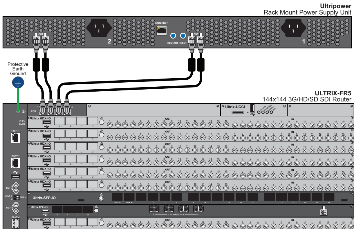
Figure 18 ULTRIX-FR5 — Power Connections
