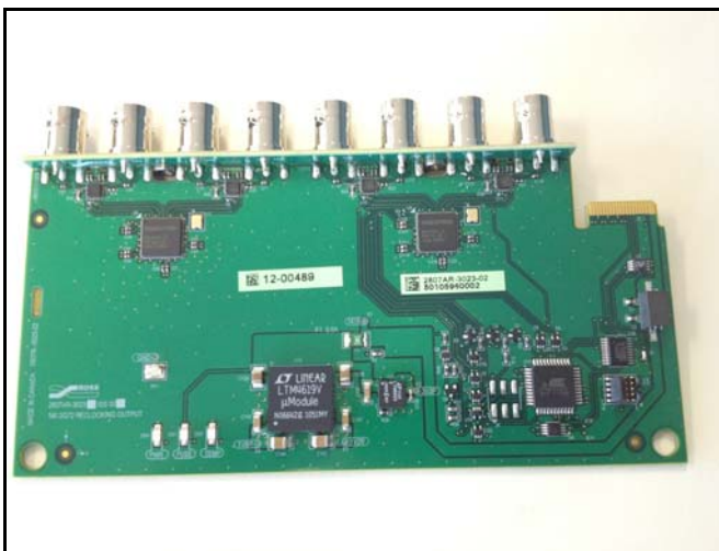
New NK-O3G72 Output Card (2807AR-3023-02, 2W)
